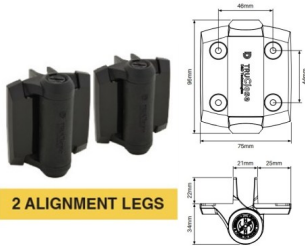
2 ALIGNMENT LEGS
