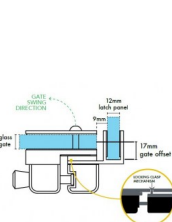
Latch Holes on Gate Panel
