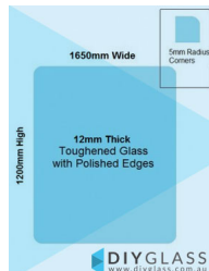
1650 x 1200mm Glass Pool Fence or Balustrade Panel
