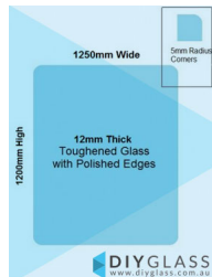
1250 x 1200mm Glass Pool Fence or Balustrade Panel
