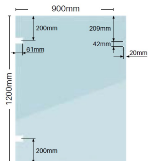
Suits glass to wall/post installation
