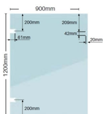
Suits glass to wall/post installation
