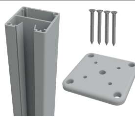
50x50mm Friction Fit Post with Base Plate and 12Gx50mm countersunk screws
